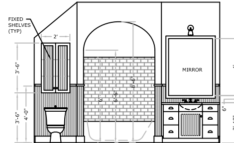
16 A5.02 2ND FLOOR BATH WOOD SPECIES: BIRCH FINISH: PAINT
