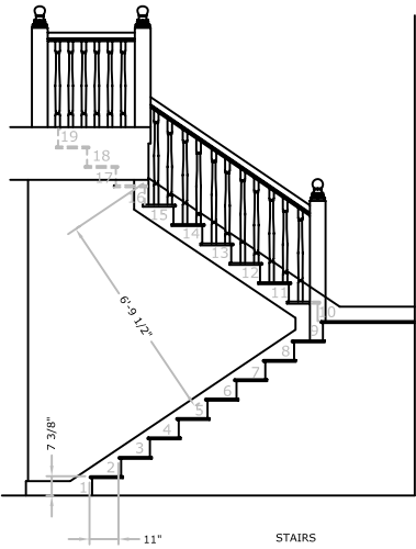
STAIRS WOOD SPECIES: PINE OR OAK FINISH: STAIN
