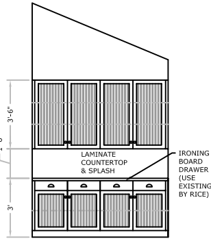
13 A5.01 LAUNDRY ROOM WOOD SPECIES: BIRCH FINISH: PAINT
