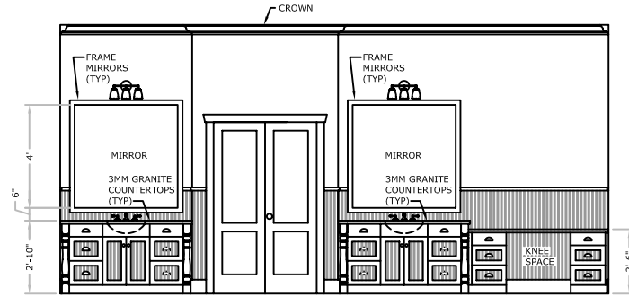
14 A5.01 MASTER BATH WOOD SPECIES: BIRCH FINISH: PAINT
