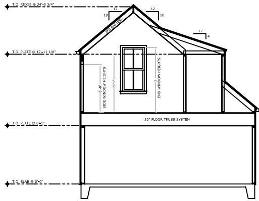
5 BUILDING SECTION THRU GARAGE A5.01
