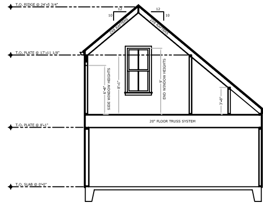
6 BUILDING SECTION THRU GARAGE A5.01
