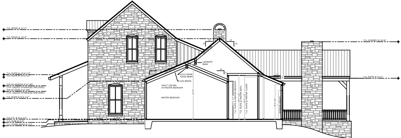
3 BUILDING SECTION THRU MASTER BEDROOM A5.01
