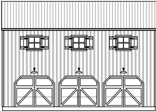
NORTH ELEVATION
