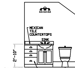
7 1ST FLOOR BATH @ SINK AS.01 WOOD SPECIES: BIRCH FINISH PAINT
