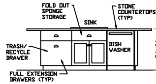
3 KITCHEN @ SINK AS.01 WOOD SPECIES: BIRCH FINISH PAINT
