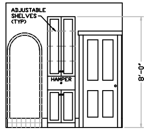
6 2ND FLOOR BATH @ LINENS AS.01 WOOD SPECIES: BIRCH FINISH PAINT
