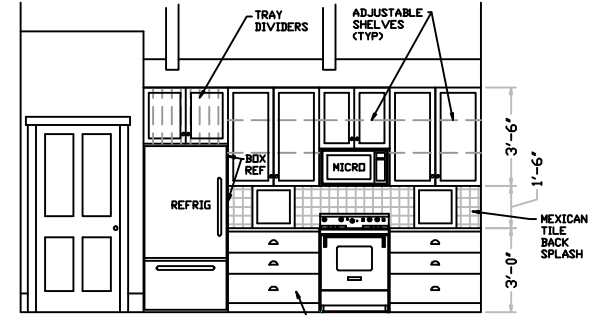
2 KITCHEN @ RANGE/REFRIGERATOR AS.01 WOOD SPECIES: BIRCH FINISH PAINT
